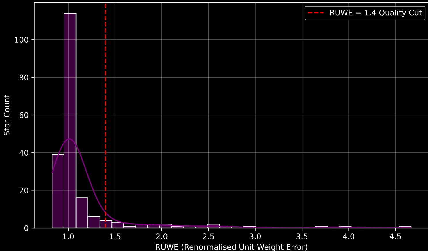
GAPOGEE DR17 Field [K2_C5_214+27_btx] RUWE Distribution (n= 198)
