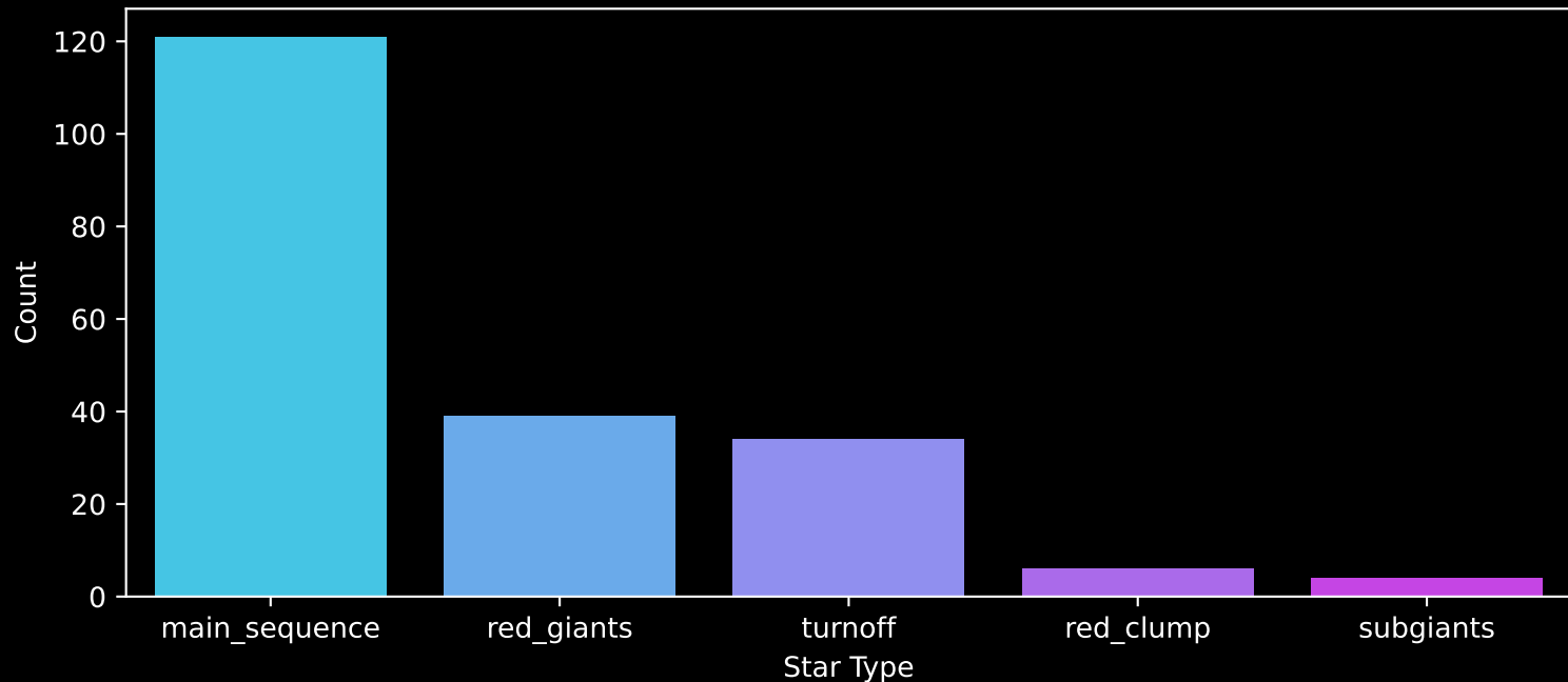
APOGEE DR17 Field: [K2_C5_214+27_btx] Count plot of Star Type
