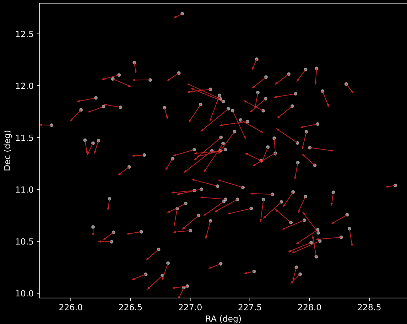
APOGEE DR17 Cluster 6 Proper Motion Vectors (n=101)
