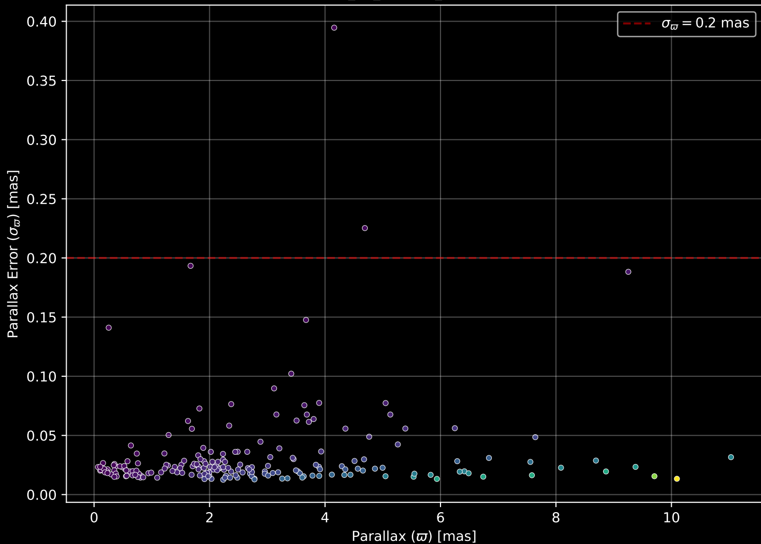
APOGEE DR17 Field: [K2_C5_214+27_btx] Parallax Quality (n= 204)
