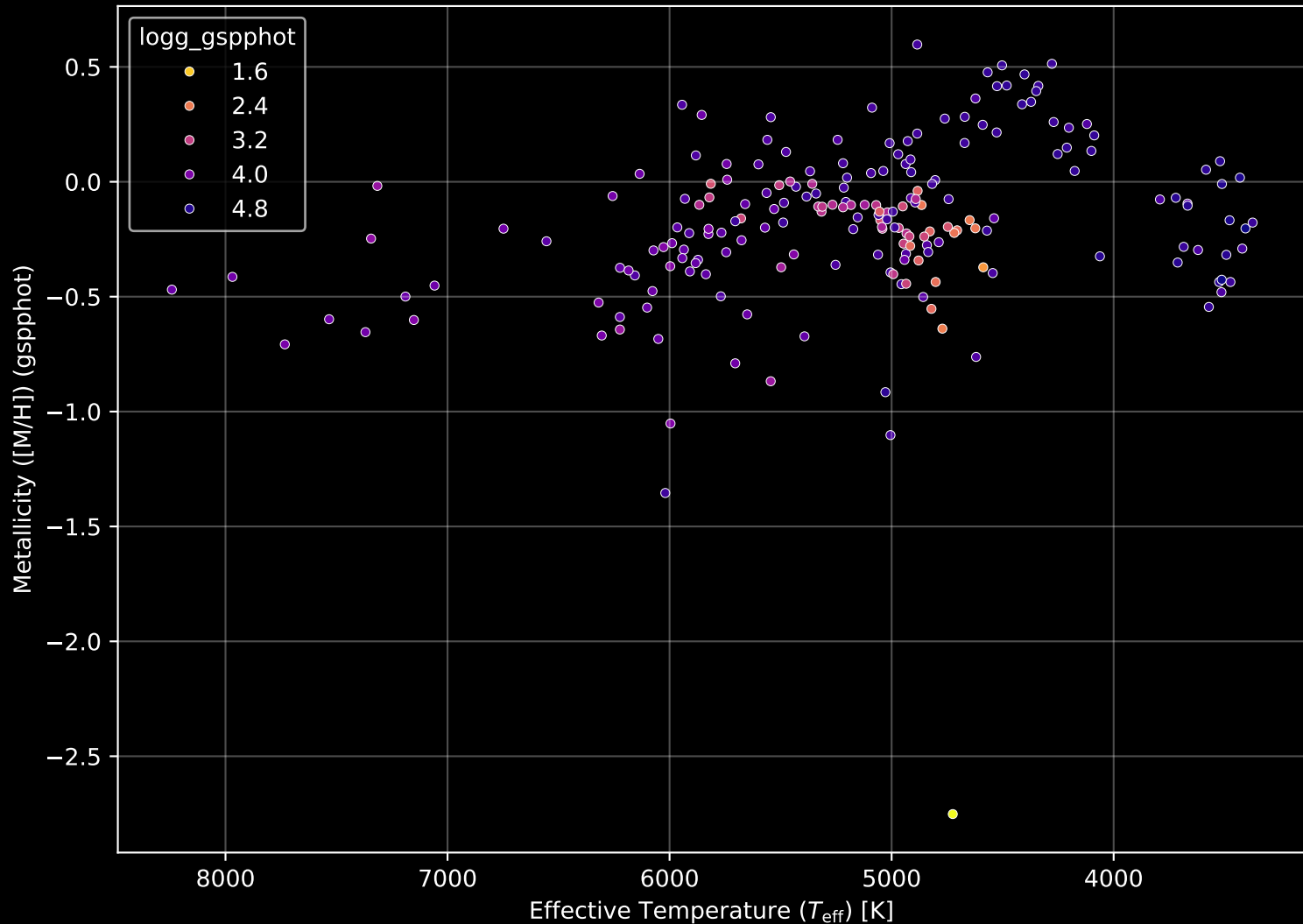
APOGEE DR17 Field: [K2_C5_214+27_btx] Stellar Population Parameters (n= 204)
