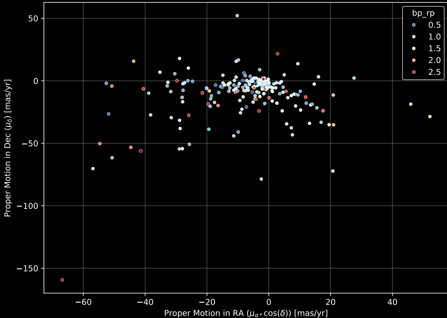
APOGEE DR17 Field: [K2_C5_214+27_btx] Proper Motion Diagram (n= 204)
