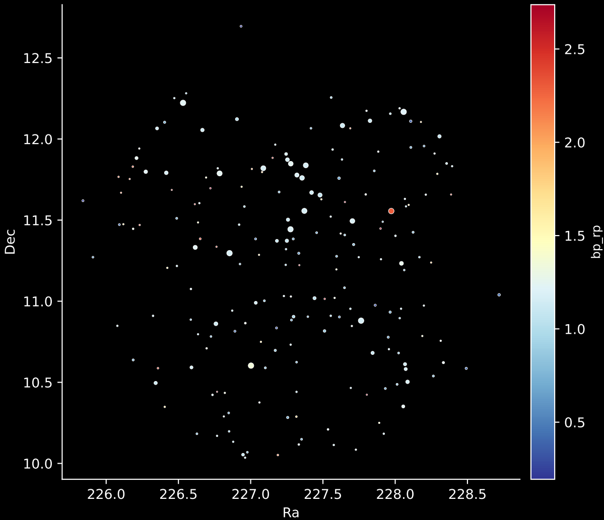
APOGEE DR17 Field: [K2_C5_214+27_btx] Stars: 204
