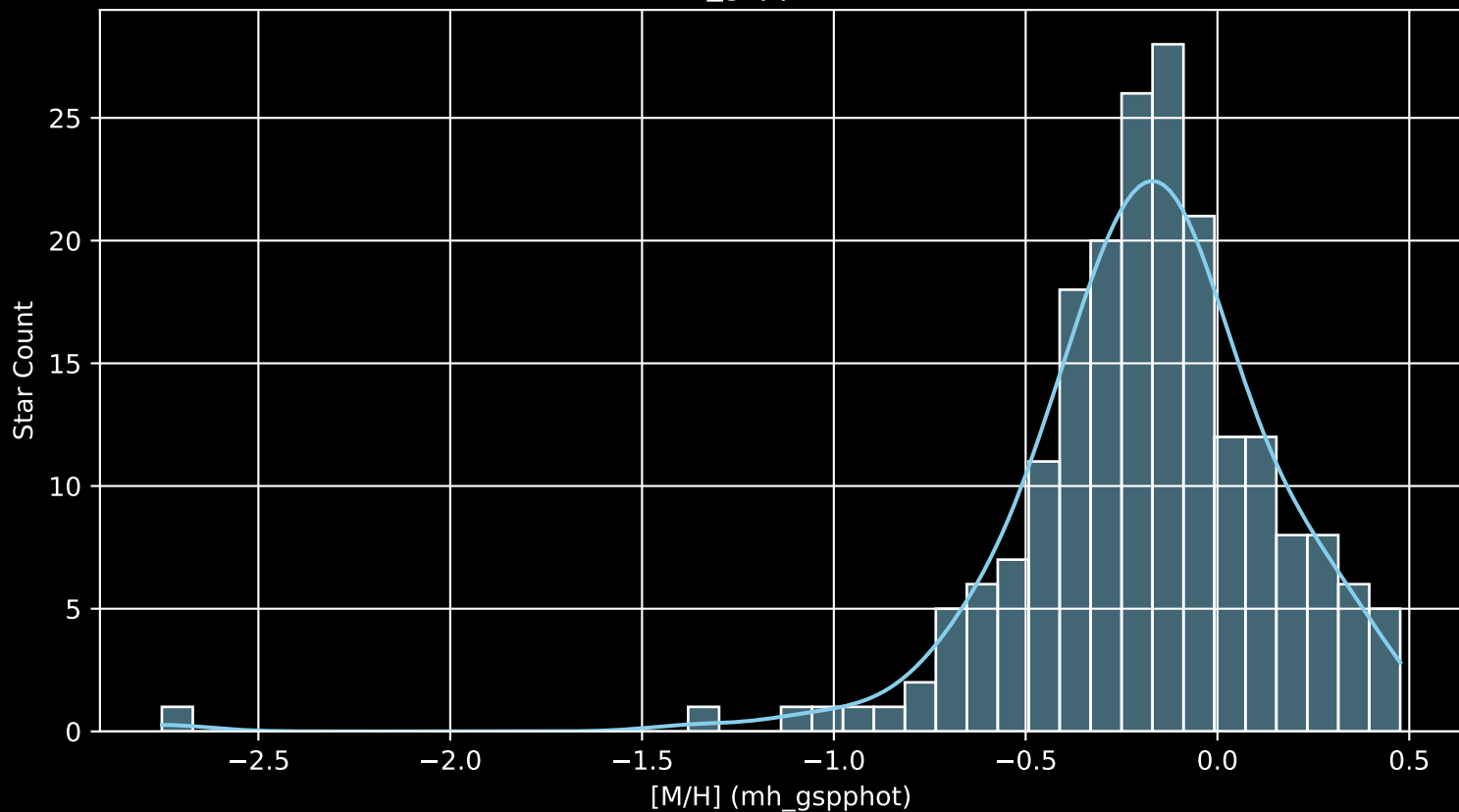
APOGEE DR17 Field: [K2_C5_214+27_btx [M/H] (mh_gspphot) (n= 201)
